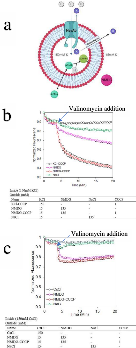
Figure 3.1. Functional characterization of the NavAb proteins by liposome flux assay. (a) Cartoon illustration of the liposome fluorescence flux assay to determine channel activities of the NavAb channels (created with BioRender.com). (b) Proton and sodium uptake via the NavAb WT channel in liposomes, driven by K + Nernst potential. Ionic conditions were listed in the table below. (c) Proton and sodium uptake via the NavAb WT channel in liposomes driven by Cs + Nernst potential. Ionic conditions were listed in the table below. The data is presented as mean \pm ste, n=3.
