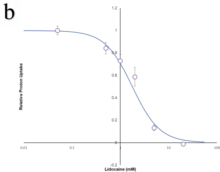
Figure 3.2. Lidocaine block of the NavAb channel. (a) Block of the proton uptake via the NavAb channel by lidocaine; (b) Dose-dependent inhibition of the proton uptake via the NavAb channel by lidocaine fitted by Hill equation. The data is presented as mean \pm ste, n=3.
